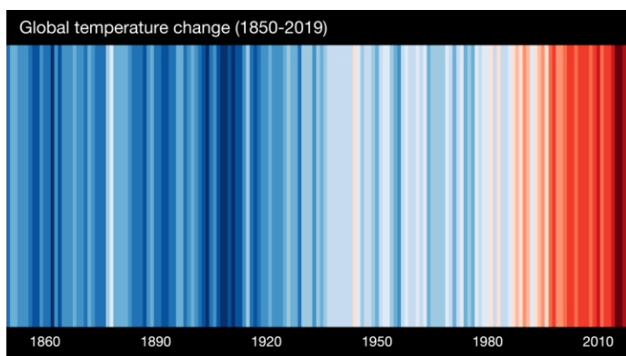
Figure 17. Global warming stripes (Hawkins, 2020 )
