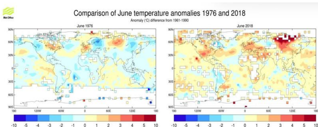
Figure 15. Comparison of 1976 and 2018 June temperature anomalies, based on Met Office Had-CRUT4 data set ( “Summer temperature 2018 – the ‘new normal’?”, 2020 – section 8 References )
