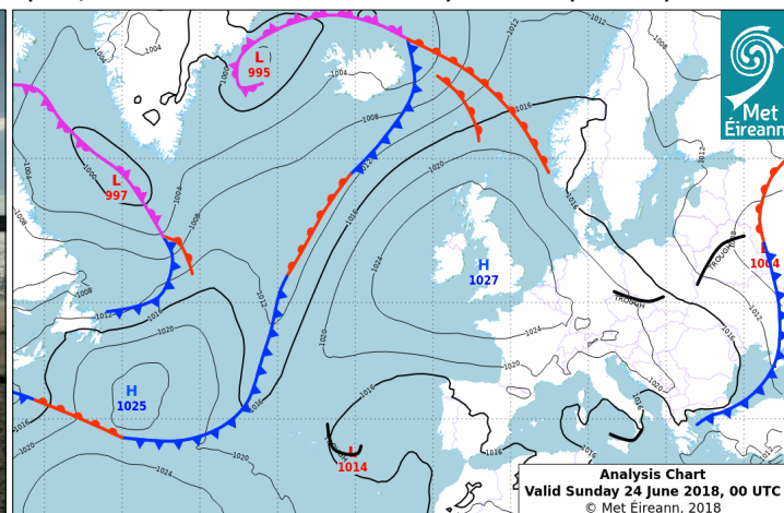
Figure 3 Surface analysis 00UTC 24th June 2018 Met Éireann
