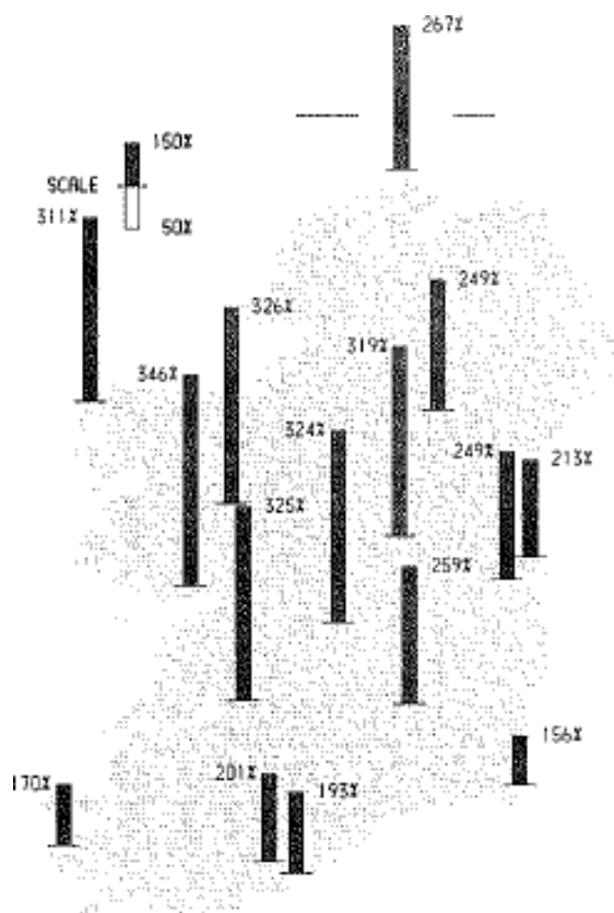
Rainfall percentage of 1951 - 1980 normals
