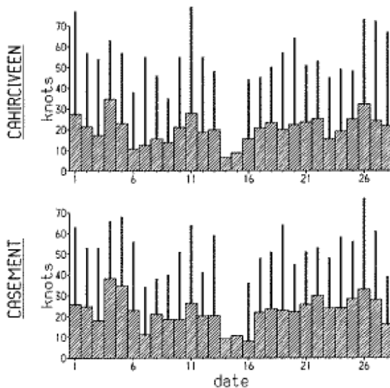
WIND SPEEDS : Daily mean speed and maximum gusts in knots
