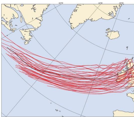
Figure 6 : ECMWF ensemble forecast tracks of possible deep depressions impacting on Ireland (actual Darwin storm track in black) (a) forecasts from 08 February 12:00 UTC
