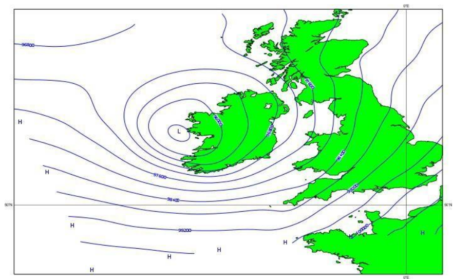
Figure 8 : HARMONIE MSLP 24 hour forecast for 12:00 UTC 12 February (b): the corresponding observed /analysis of MSLP.
