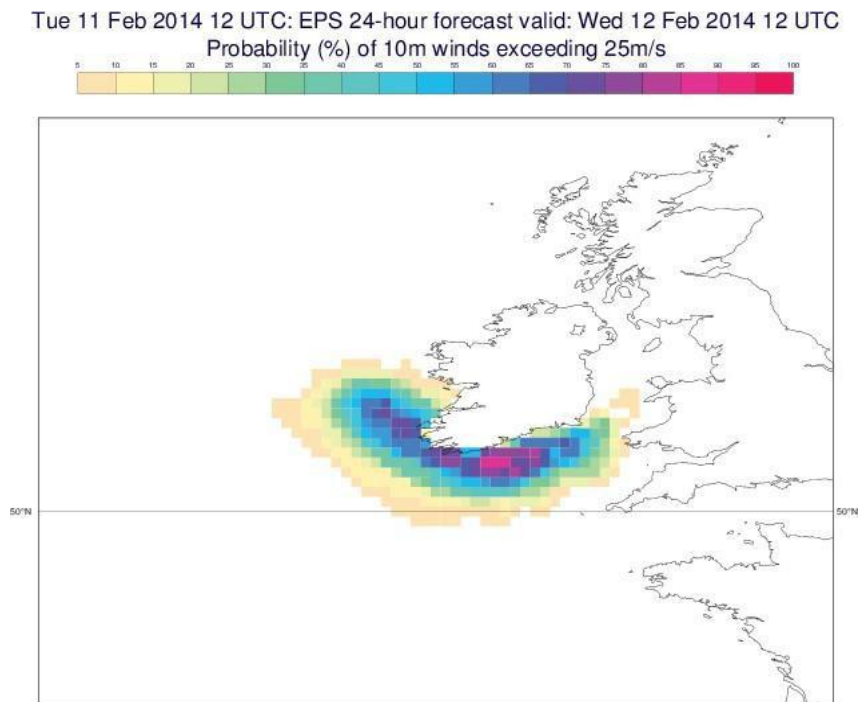
Figure 7 (b): ECMWF ensemble forecasts valid for 12:00 UTC 12 February for (b) 24-hour forecast of the probability of winds exceeding 25 m/s.
