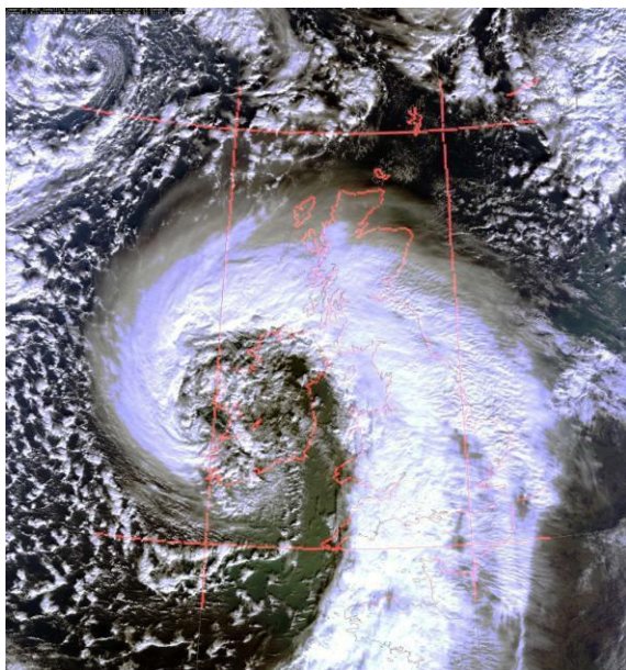
Figure 1 (a): RGB composite satellite image from the Moderate Resolution Imaging Spectroradiometer (MODIS) on NASA's Terra satellite for 11:45 UTC 12 February, 2014 (NASA, 2014; Dundee Satellite Receiving Station, 2014).
