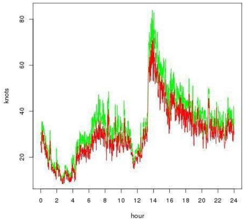
Figure 2 (a): Mace Head minute resolution wind trace (green curve: gusts; red curve: 10-minute winds)
