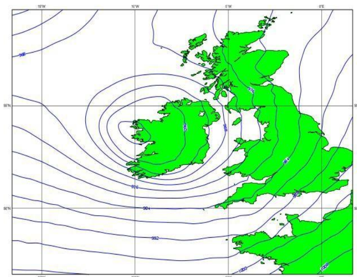
Figure 1 (b): Mean sea level pressure analysis for 12:00 UTC.
