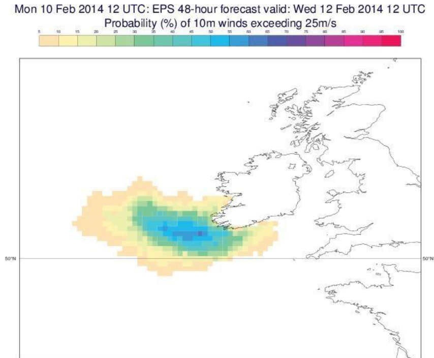
Figure 7 (a): ECMWF ensemble forecasts valid for 12:00 UTC 12 February for (a) 48-hour forecast of the probability of winds exceeding 25 m/s
