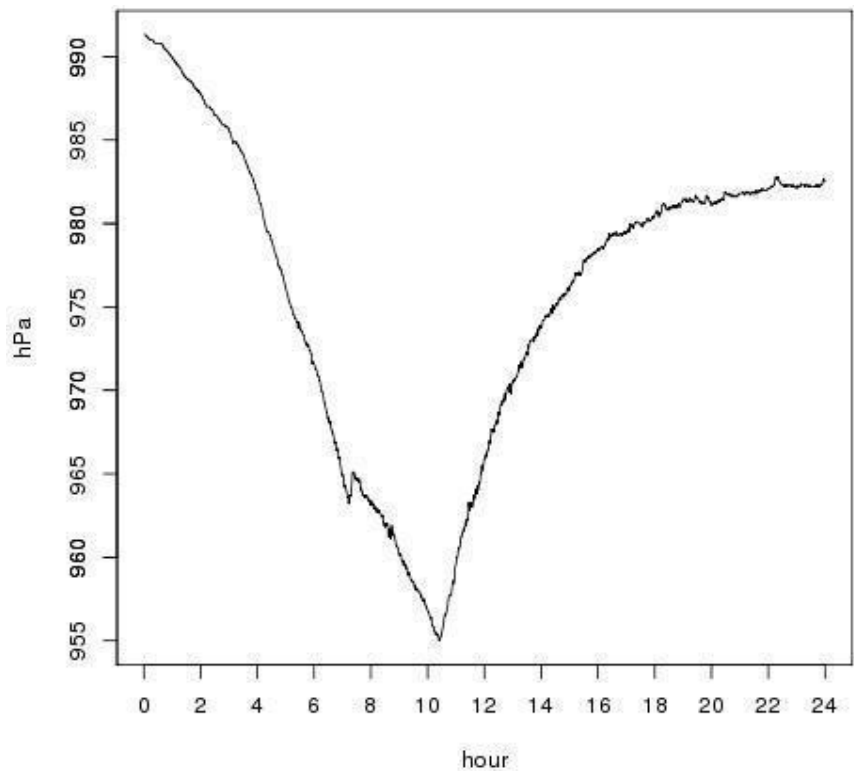
Figure 2 (b) Valentia Observatory pressure trace for 12 February, 2014
