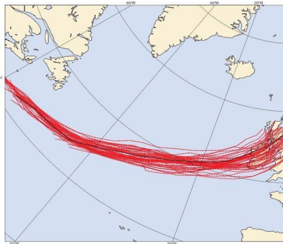
Figure 6 (b): ECMWF ensemble forecast tracks of possible deep depressions impacting on Ireland (actual Darwin storm track in black) forecasts from 10 February 00:00 UTC. The spread in the tracks is indicative of the forecasts.
