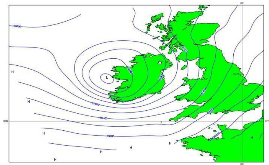
Figure 8 (a): HARMONIE MSLP 24 hour forecast for 12:00 UTC 12 February
