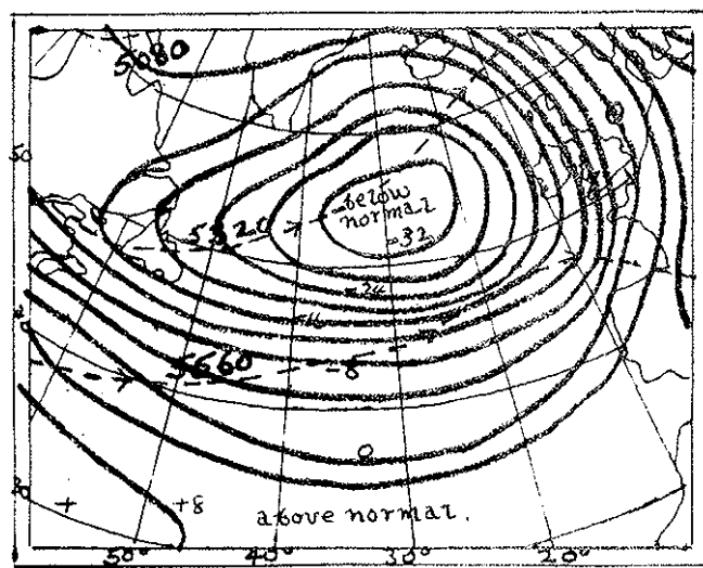
(b) 500mb anomalies in 4mb intervals. Dashed lines indicate the normal flow for January.
