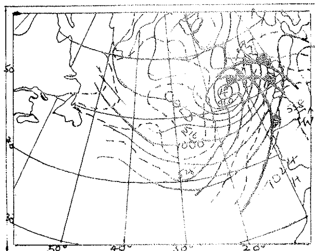
(b) 120000z: Surface synoptic (solid lines) and 1000/500 thickness analysis (dashed lines) in dm.
