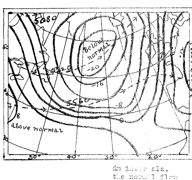
(b) 500mb anomalies in 4 dm intervals. Dashed lines indicate the normal flow for January.
