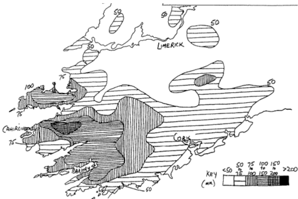
Rainfall mm for the 24-hour period beginning 10AM on 5th August
