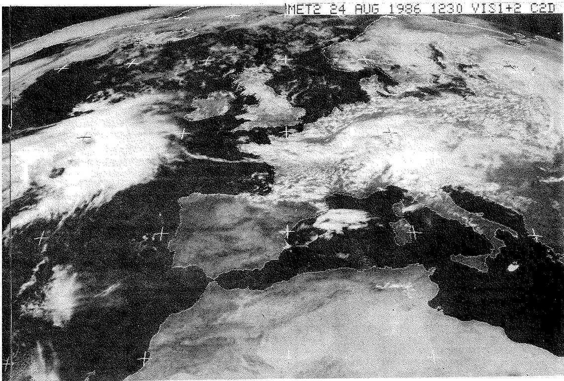
Hurricane Charley and the storm of the 25th
