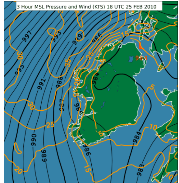
Weather chart with isobars, 25 Feb 2010
